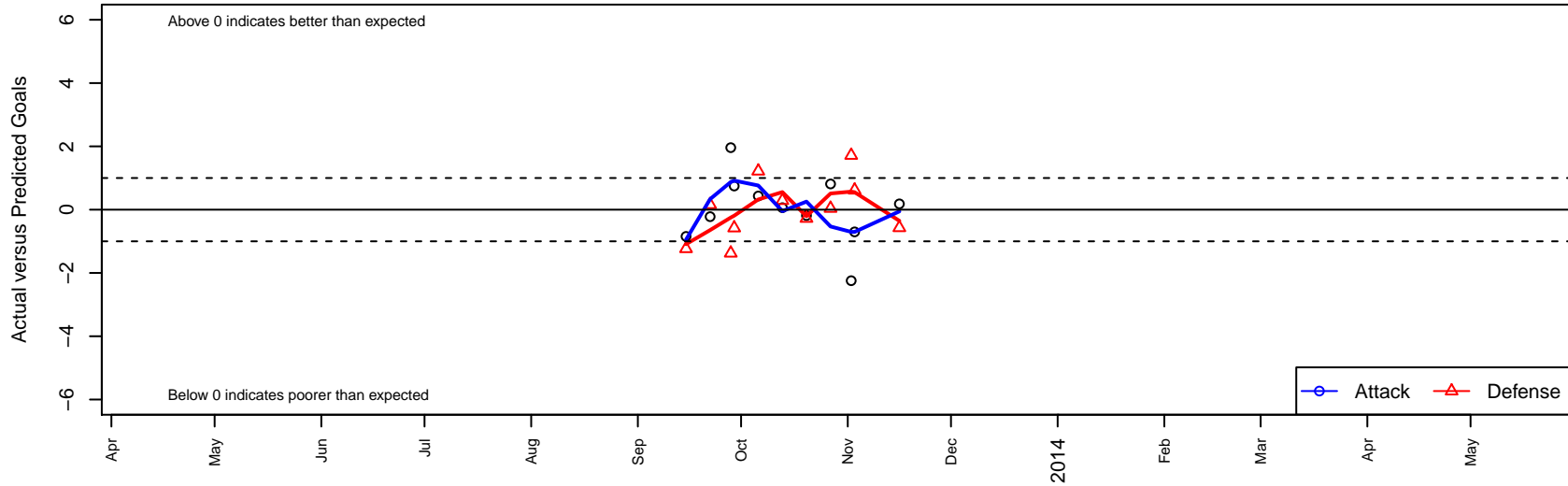
Exiles SC Black B94 Dots are actual minus expected GF (blue circles) and GA (red triangles). Blue line is smoothed change in attack strength. Red is smoothed change in defense strength.
